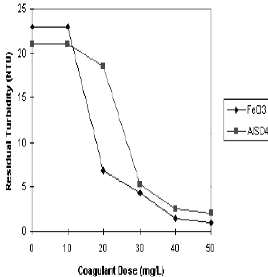
Water B Coagulant Dose vs. Residual Turbidity
